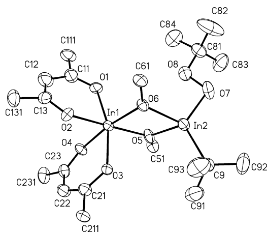
Figure 2. Molecular structure and numbering scheme of 3 ; the thermal ellipsoids are drawn at the 40% probability level; hydrogen atoms and the methyl groups of the tert -butoxy bridges and acetylacetonato ligands are omitted. Selected bond lengths [pm] and angles ^\circ : In1–O1 213.2(4), In1–O2 215.1(4), In1–O3 214.8(4), In1–O4 216.0(4), In1–O5 213.3(4), In1–O6 214.0(4), In2–O5 213.0(4), In2–O6 212.4(4), In2–O7 202.8(5), In2–C9 221.0(7), O7–O8 149.0(7), In2–O7–O8 102.2(3), O7–O8–C81 107.9(5).
