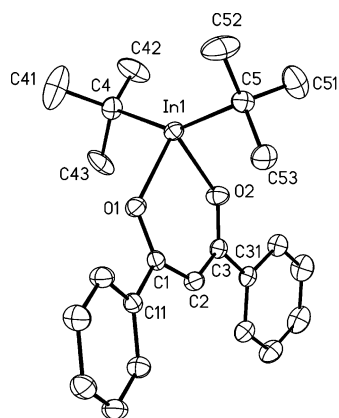
Figure 1. Molecular structure and numbering scheme of 2 ; the thermal ellipsoids are drawn at the 40% probability level; hydrogen atoms are omitted. Selected bond lengths [pm] and angles [°]: In1–C4 218.3(2), In1–C5 217.6(2), In1–O1 215.3(2), In1–O2 218.3(2), O1–In1–O2 84.38(6), C4–In1–C5 148.29(8).
