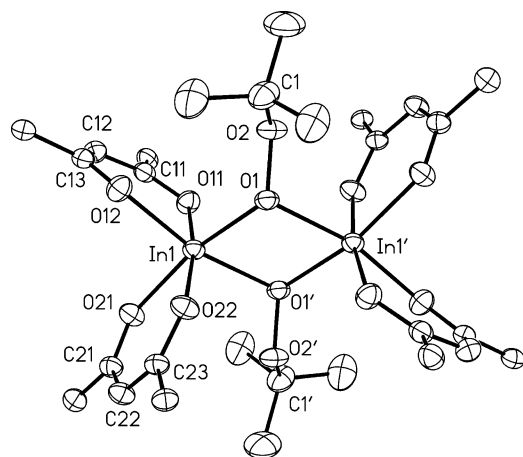
Figure 3. Molecular structure and numbering scheme of 4 ; the thermal ellipsoids are drawn at the 40% probability level; hydrogen atoms and phenyl groups are omitted. Selected bond lengths [pm] and angles [°]: In1–O11 213.1(2), In1–O12 211.7(2), In1–O21 213.1(2), In1–O22 212.3(2), In1–O1 217.3(2), In1–O1' 215.1(2), O1–O2 147.0(3), In1–O1–O2 119.3(2), In1'–O1–O2 109.2(2), O1–O2–C1 109.3(3), In1–O1–In1' 104.3(1), O1–In1–O1' 75.8(1); In1' and O1' generated by -x + 1, -y, -z + 1 .
